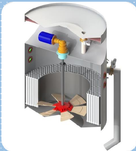
Mechanical Pan Circulators
